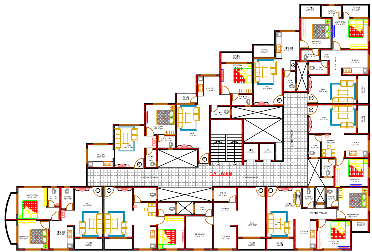
TYPICAL FLOOR PLAN - ( 1st TO 9th ) LOTUS
