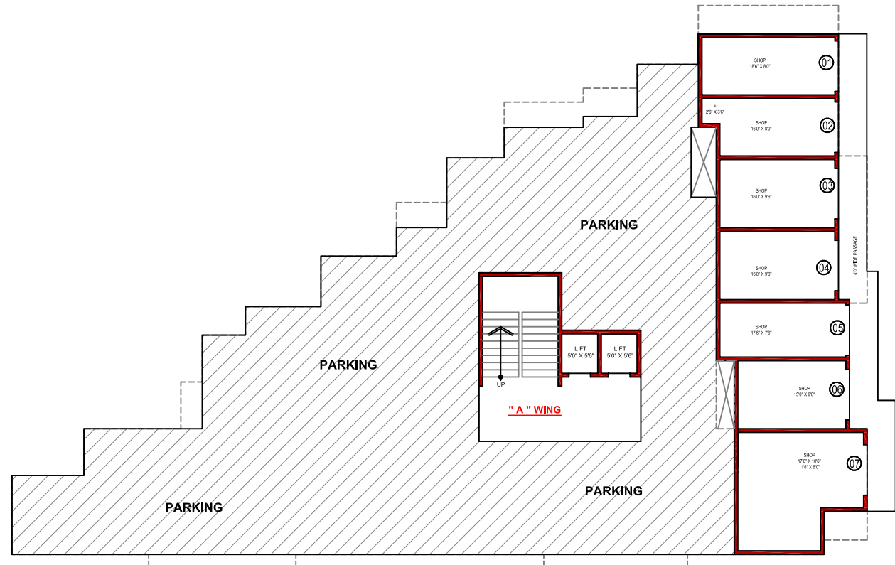
GROUND FLOOR PLAN LOTUS
